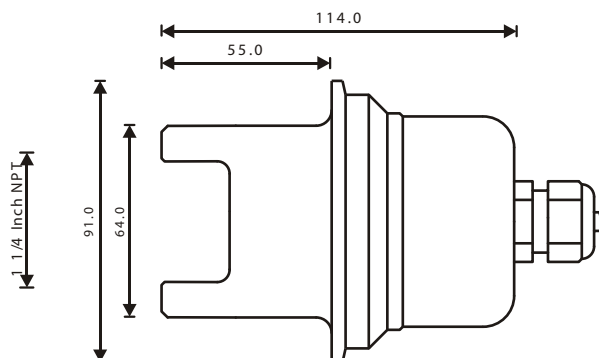
Hygienic Sensor
