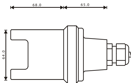
Immersion Sensor
